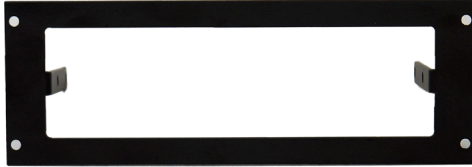
93757 Havis, Inc. Console Plate H 2.988" x W 8.594" x D 0.09"
