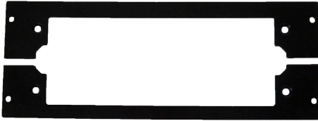
93417 Havis, Inc. Console Plate H 2.968" x W 8.594" x D 0.09"
