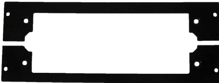
93427 Precision Mounting Technologies Console Plate H 2.968" x W 8.75" x D 0.25"
