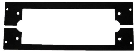
93426 D&R Electronics Console Plate H 2.98" x W 8" x D 0.09"
